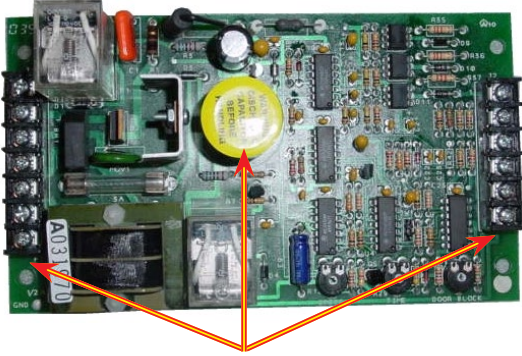
Large capacitor and terminal strips at each end
