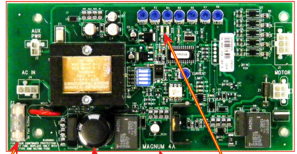
Fuse Large Capacitor Magnum 4A LEDs
