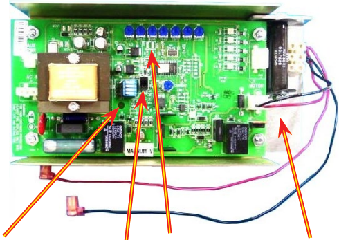
5th Mounting Hole Two Position Slide Switch LED's Brake Module
