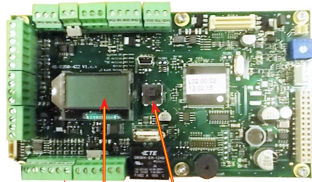
Terminal Blocks Programming Display Joystick Programming Knob
