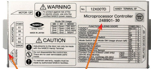
LED Indicators
