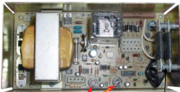
Time Adjustment Pots
