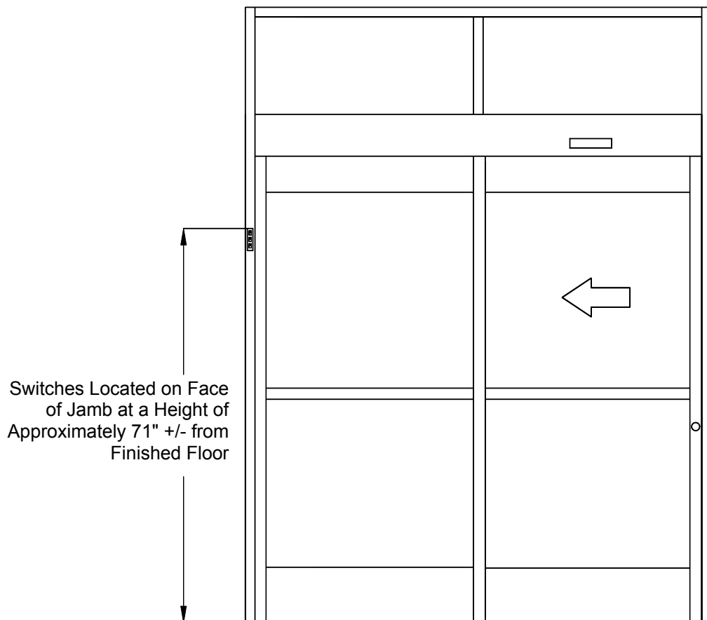
Interior Elevation (full open slider shown)
