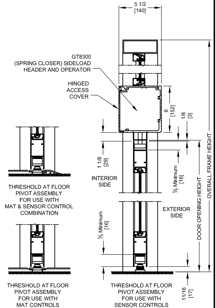
VERTICAL SECTION
