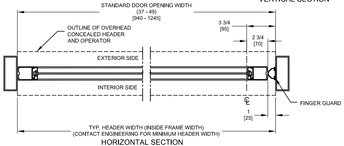
HORIZONTAL SECTION
