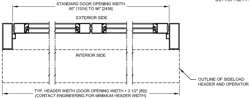
HORIZONTAL SECTION
