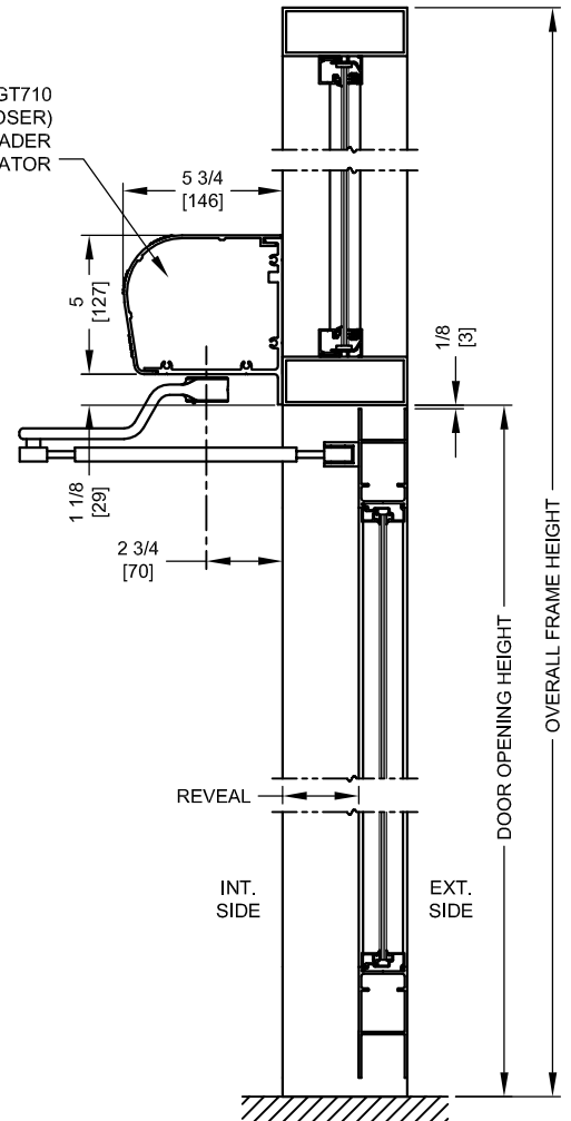
VERTICAL SECTION BUTT/OFFSET PIVOT
