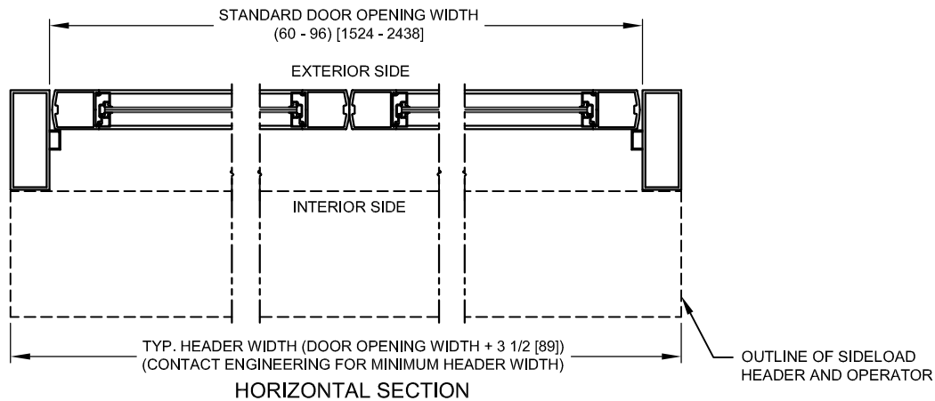
HORIZONTAL SECTION
