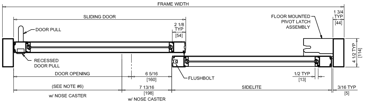
HORIZONTAL SECTION
