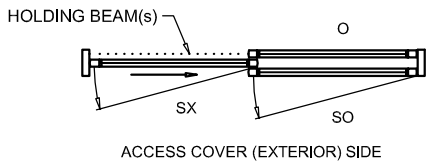
ACCESS COVER (EXTERIOR) SIDE EXTERIOR ELEVATION/PLAN
