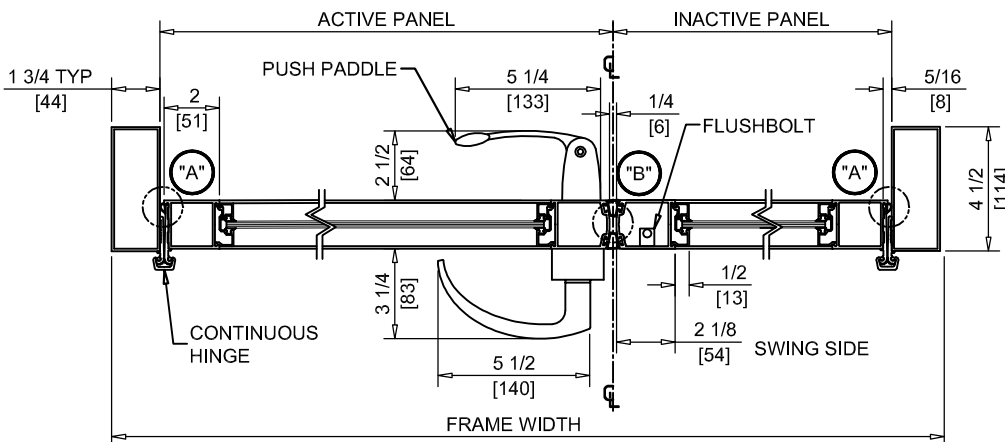
HORIZONTAL SECTION (TYPE "A")
